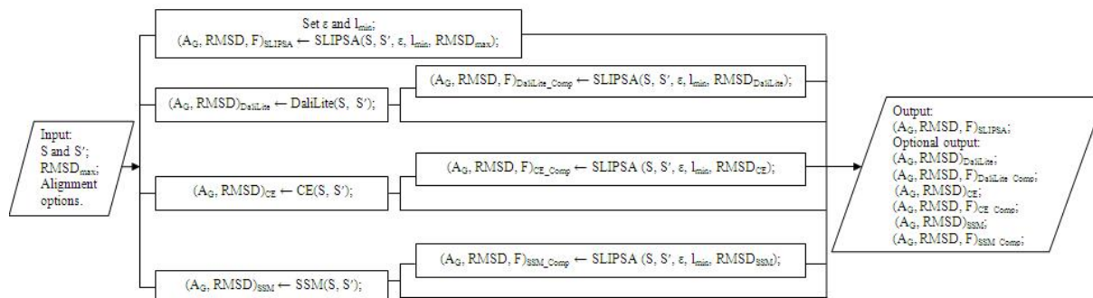
Figure 6: The web alignment work flow
